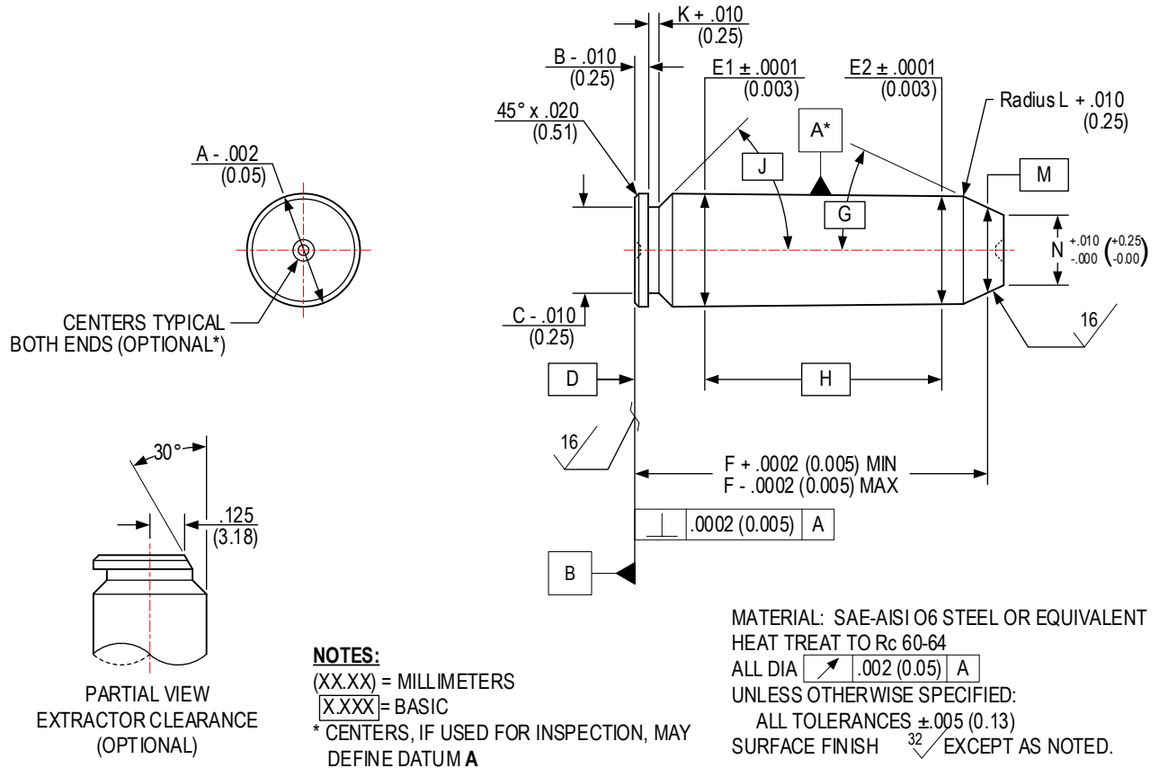
FIGURE V SHOULDER-BREACHING CENTERFIRE RIFLE HEADSPACE GAUGES (CARTRIDGE DESIGNS WITH NO INTEGRAL NECK)
