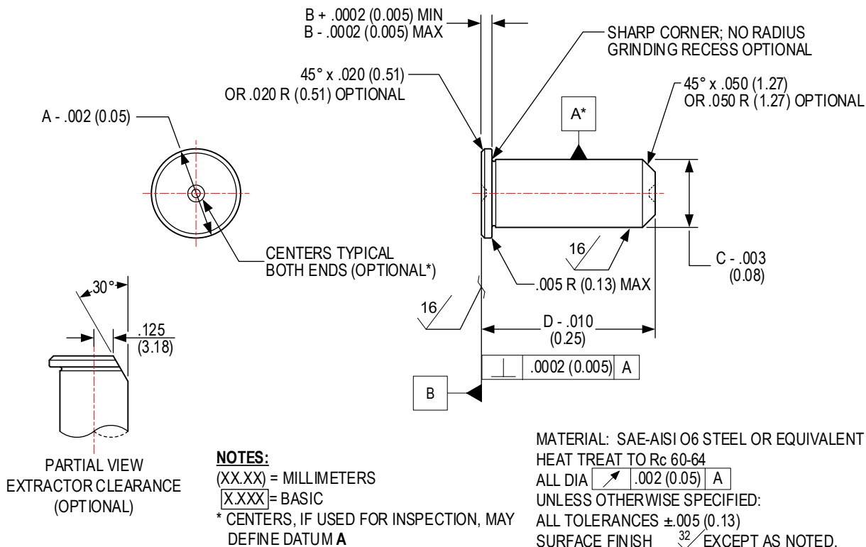
FIGURE III RIM-BREECHING CENTERFIRE RIFLE HEADSPACE GAUGES
