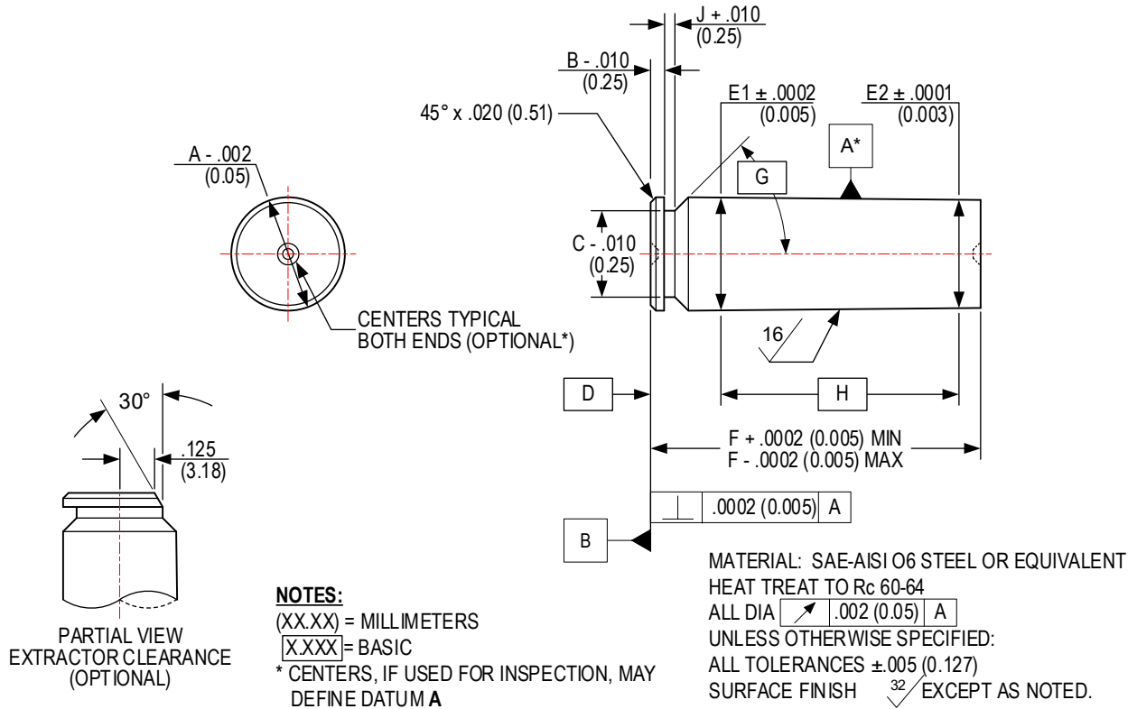
FIGURE IV MOUTH-BREACHING CENTERFIRE RIFLE HEADSPACE GAUGES
